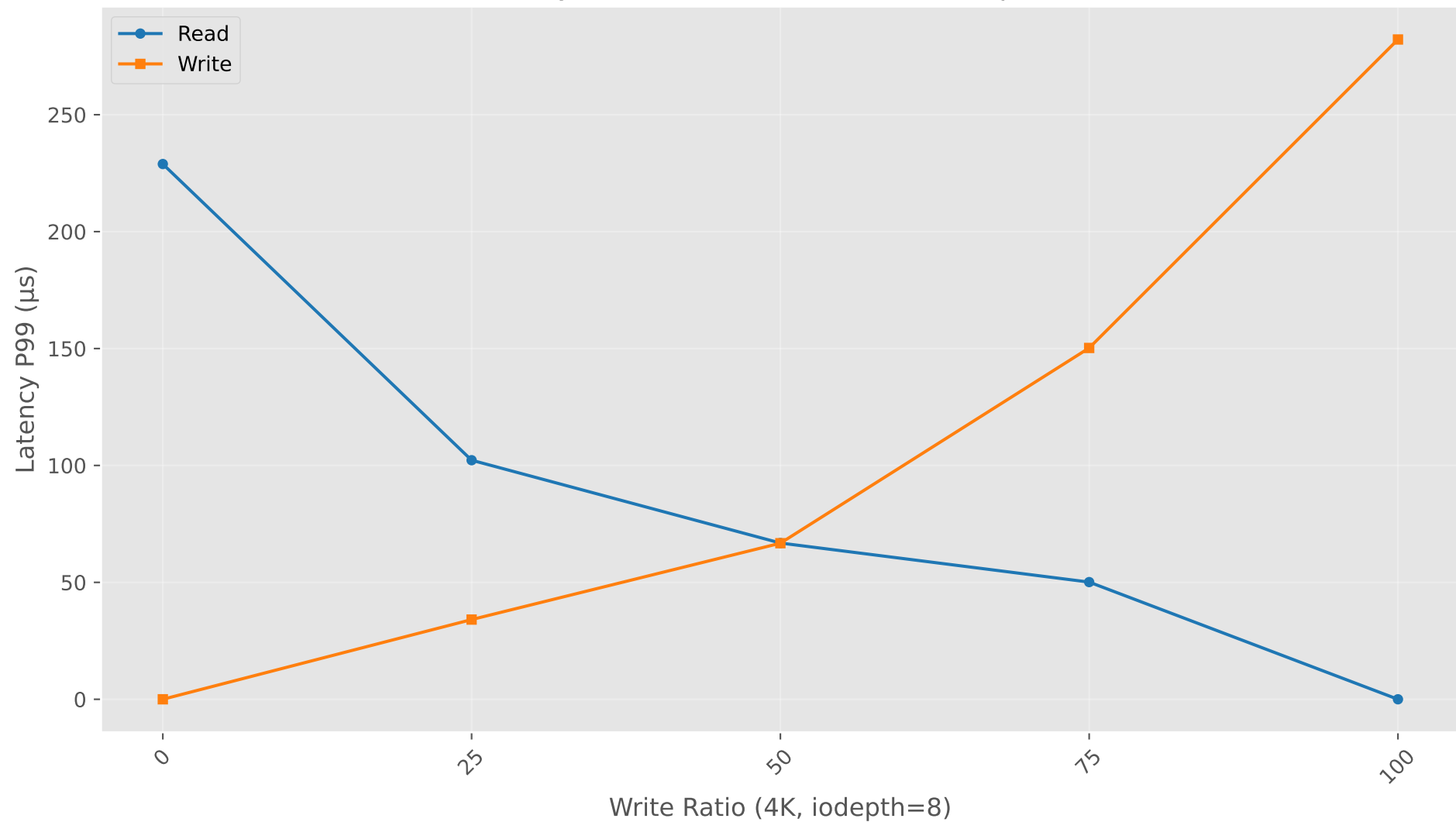
Latency P99 vs Write Ratio (4K, iodepth=8)
